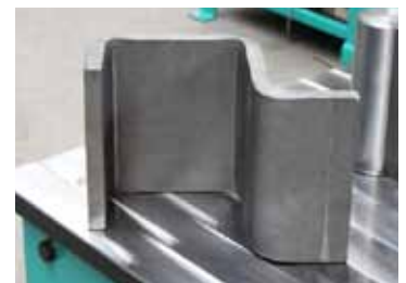
97 Dicker Flachstahl biegen Bending of thick flat steel
